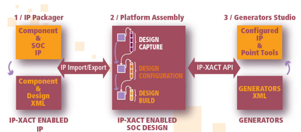
Figure 4: principle schema for an IP-XACT flow
