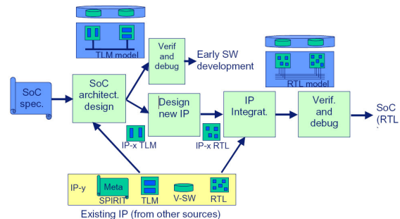
Figure 2: The SoC design flow proposed in SPRINT
